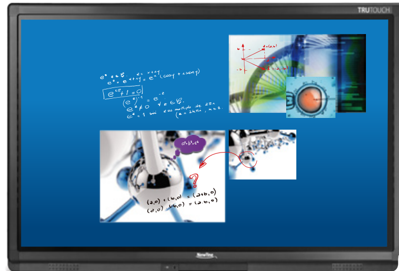
Object Projection
